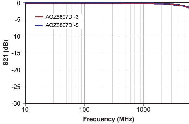
I/O - GND Insertion Loss ( S_{21} ) vs. Frequency
