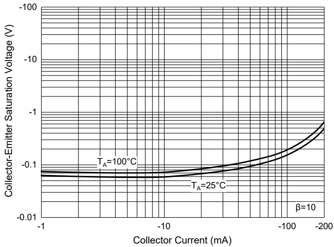
Fig. 9 - Collector-Emitter Saturation Voltage Characteristics
